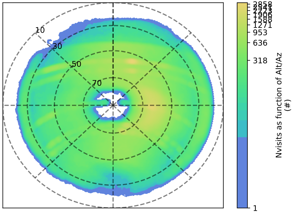
ddf_acor_sf20_lsf40_lsr50_v3.4_10yrs z: Nvisits as function of Alt/Az
