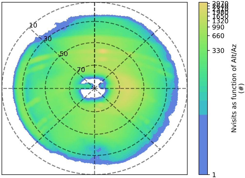
ddf_acor_sf20_lsf40_lsr50_v3.4_10yrs r: Nvisits as function of Alt/Az
