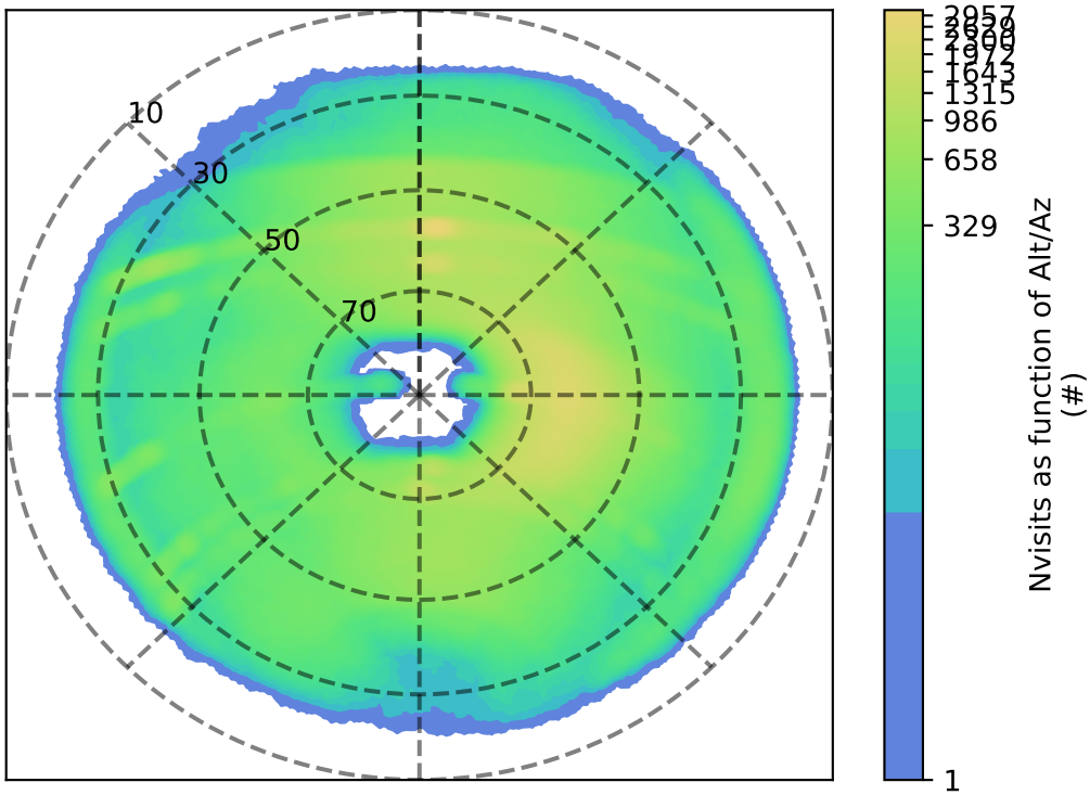
ddf_acor_sf20_lsf40_lsr50_v3.4_10yrs i: Nvisits as function of Alt/Az
