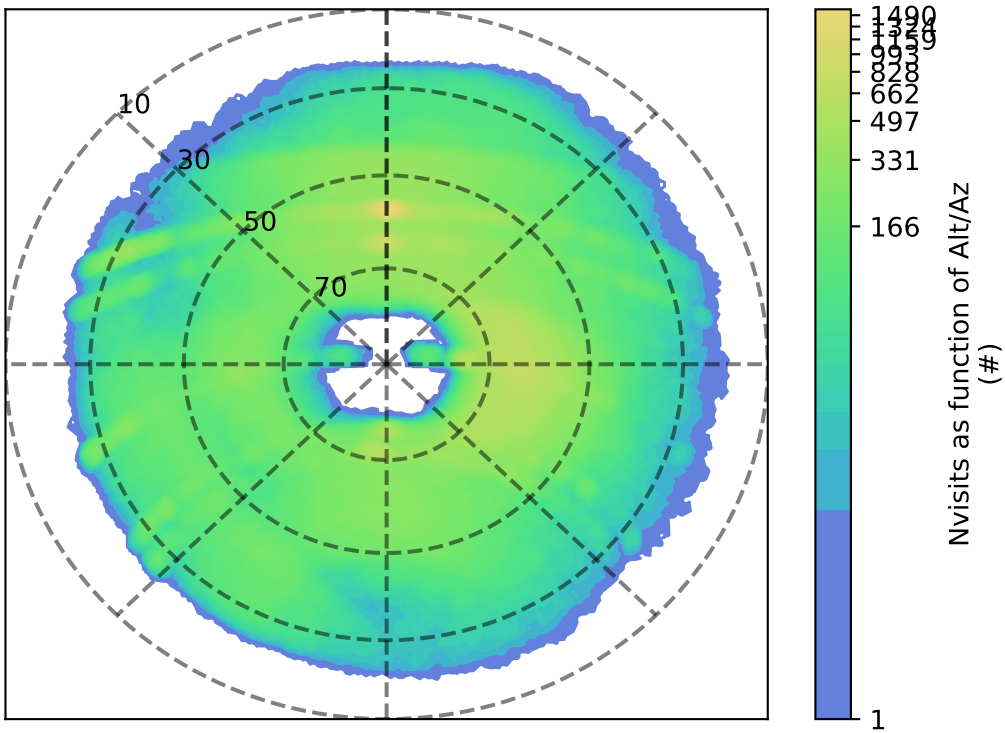
ddf_acor_sf20_lsf40_lsr50_v3.4_10yrs g: Nvisits as function of Alt/Az
