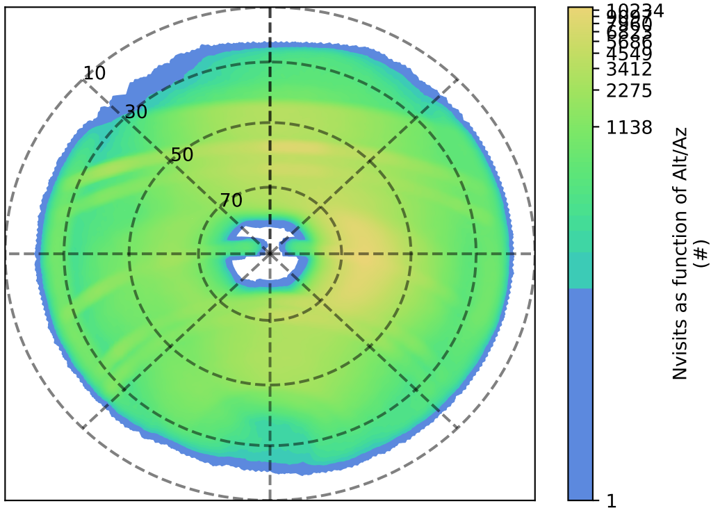
ddf_acor_sf20_lsf40_lsr50_v3.4_10yrs : Nvisits as function of Alt/Az
