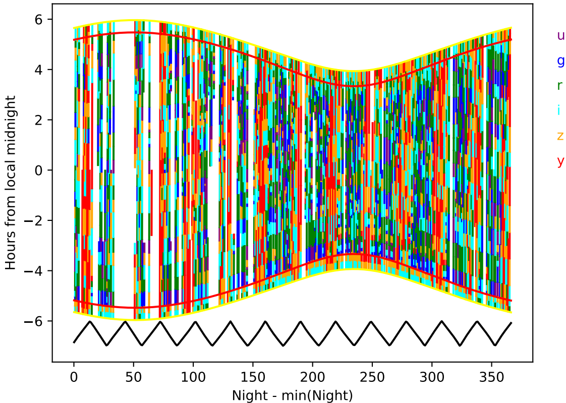
ddf_acor_sf20_lsf40_lsr50_v3.4_10yrs year 8-9: Hourglass
