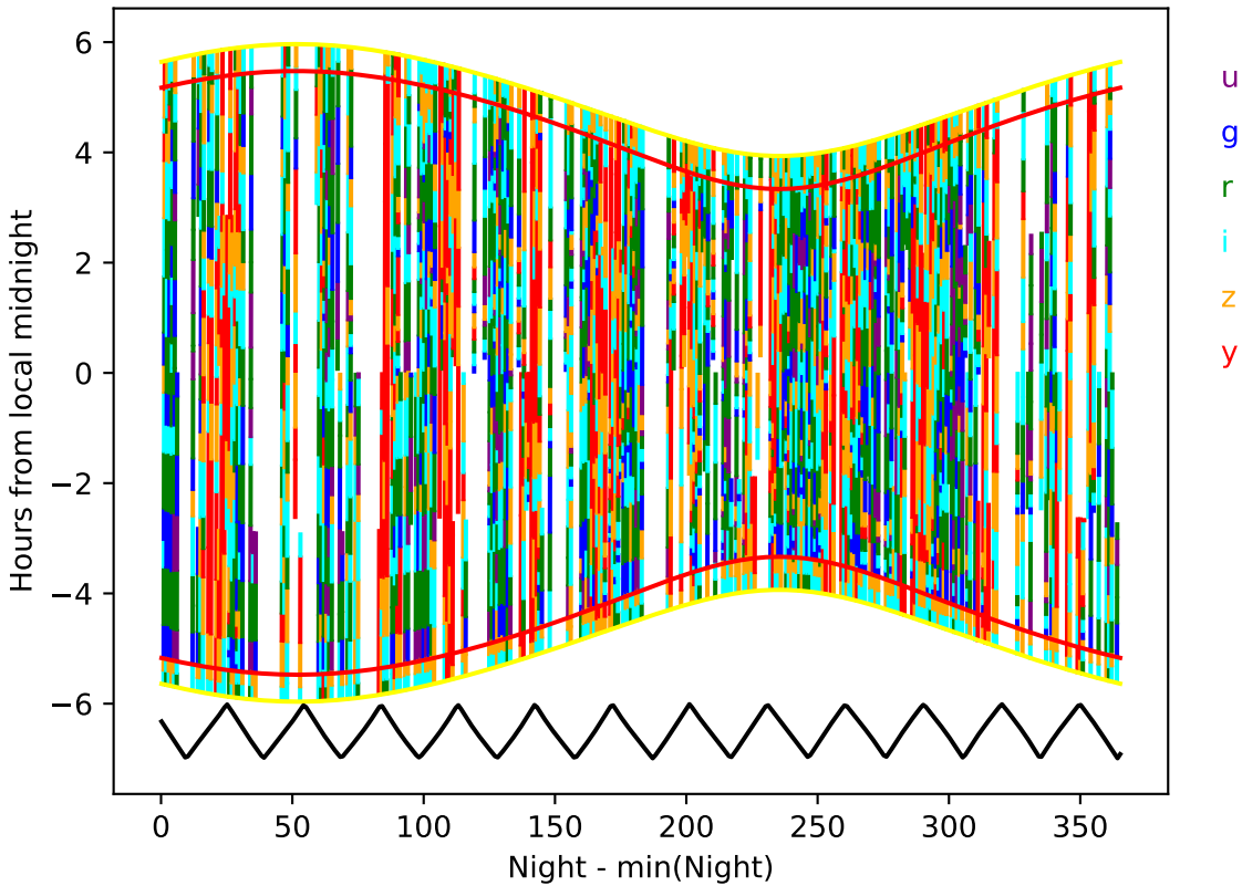
ddf_acor_sf20_lsf40_lsr50_v3.4_10yrs year 7-8: Hourglass
