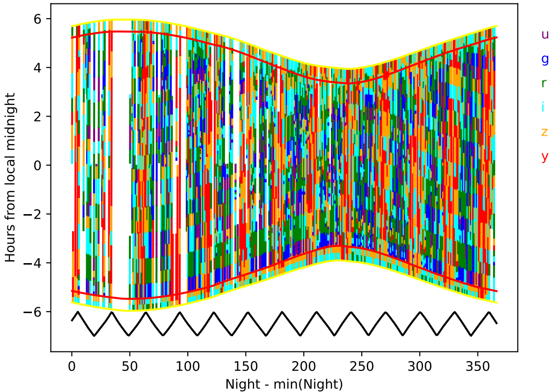
ddf_acor_sf20_lsf40_lsr50_v3.4_10yrs year 6-7: Hourglass
