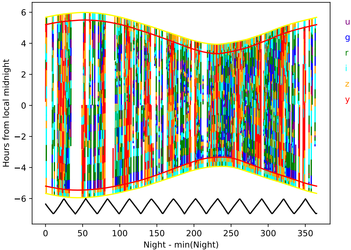
ddf_acor_sf20_lsf40_lsr50_v3.4_10yrs year 4-5: Hourglass
