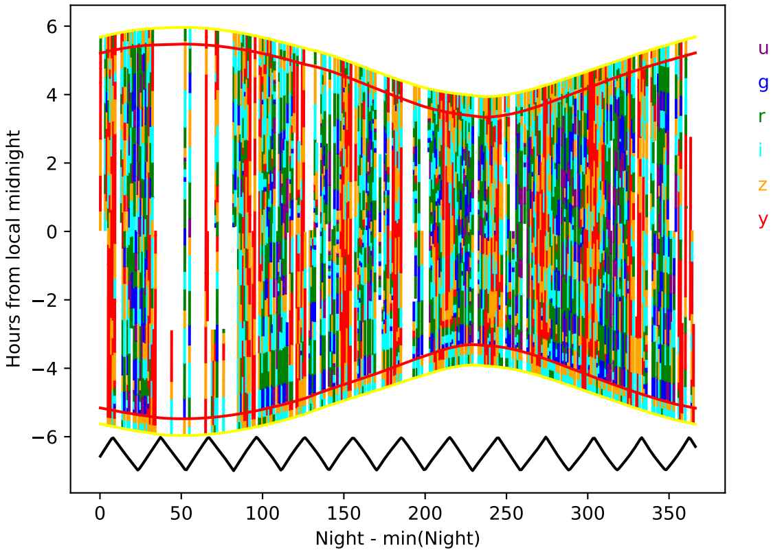
ddf_acor_sf20_lsf40_lsr50_v3.4_10yrs year 3-4: Hourglass
