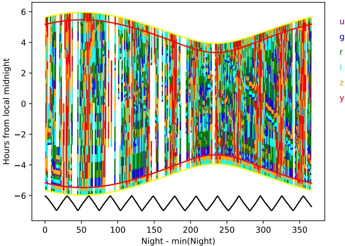
ddf_acor_sf20_lsf40_lsr50_v3.4_10yrs year 1-2: Hourglass
