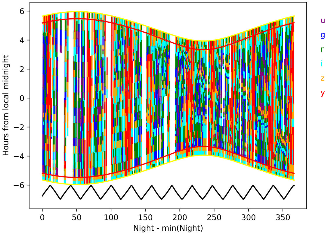
ddf_acor_sf20_lsf40_lsr50_v3.4_10yrs year 0-1: Hourglass
