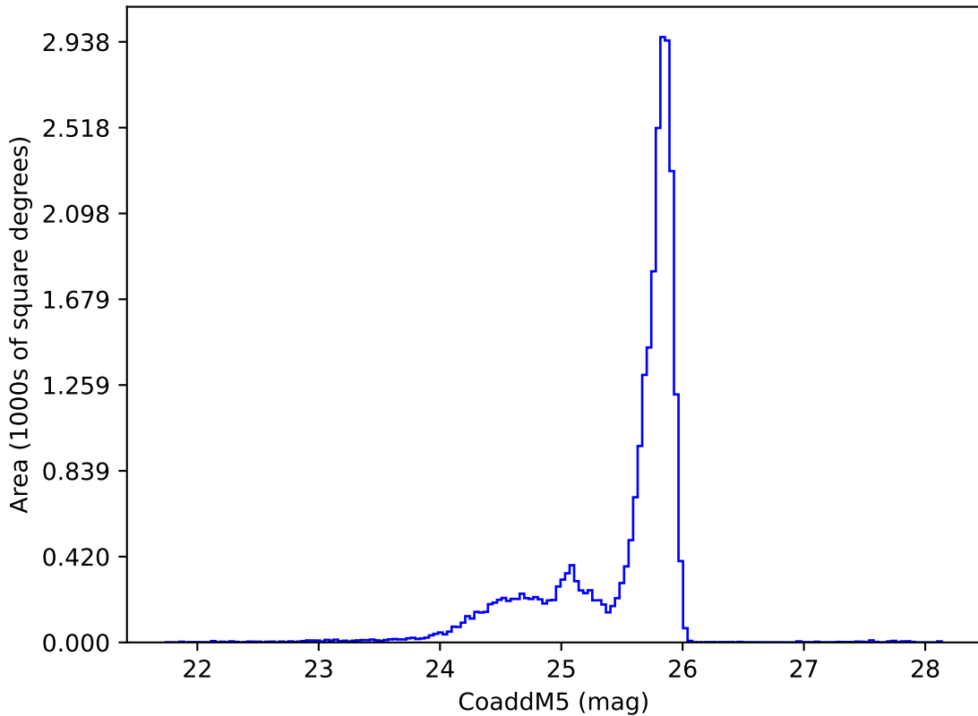
ddf_acor_sf20_lsf40_lsr50_v3.4_10yrs z: CoaddM5
