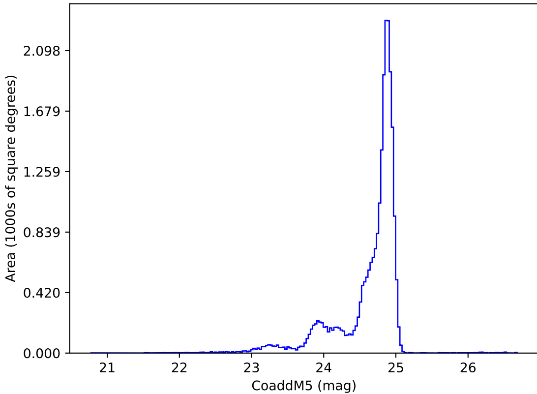
ddf_acor_sf20_lsf40_lsr50_v3.4_10yrs y: CoaddM5
