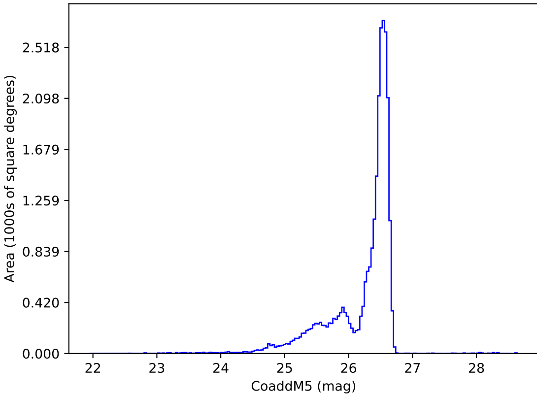
ddf_acor_sf20_lsf40_lsr50_v3.4_10yrs i: CoaddM5
