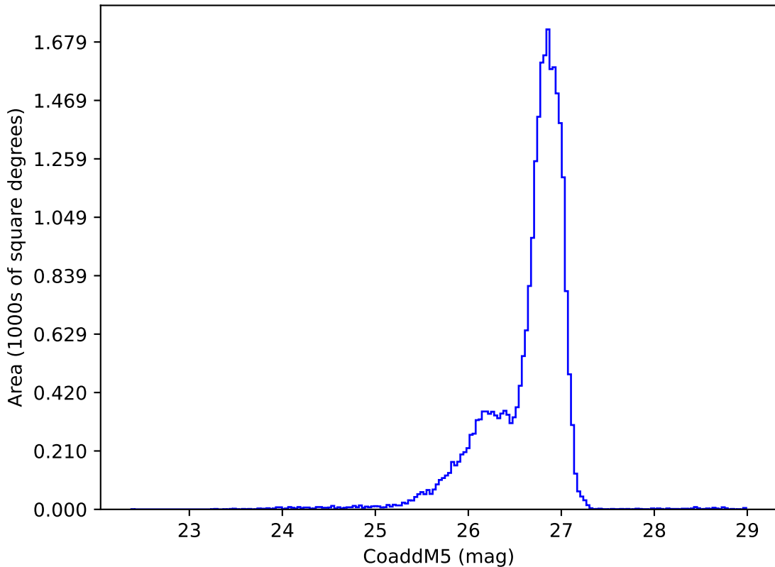
ddf_acor_sf20_lsf40_lsr50_v3.4_10yrs g: CoaddM5
