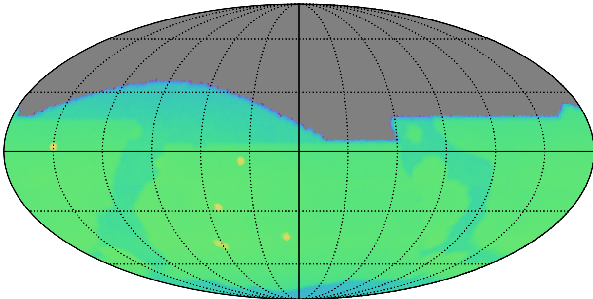
ddf_acor_sf20_lsf40_lsr50_v3.4_10yrs : CoaddM5
