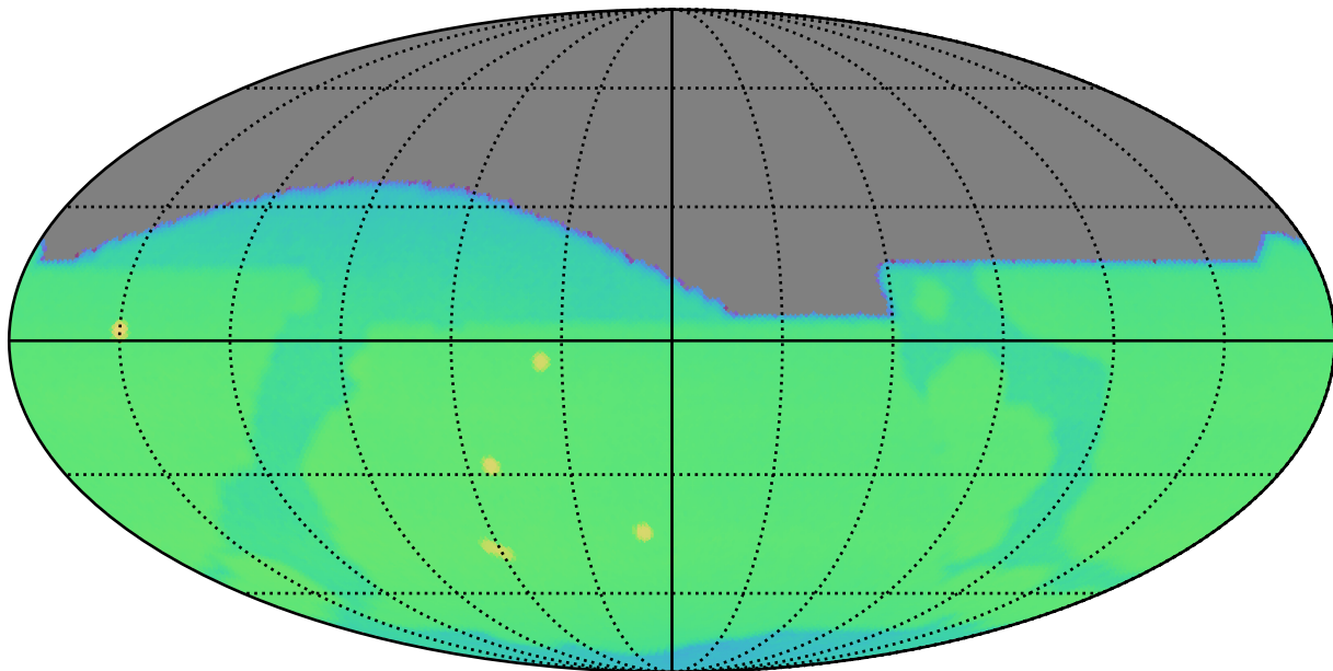
ddf_acor_sf20_lsf40_lsr50_v3.4_10yrs : CoaddM5
