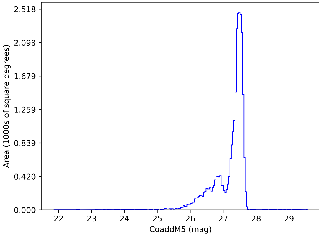
ddf_acor_sf20_lsf40_lsr50_v3.4_10yrs : CoaddM5
