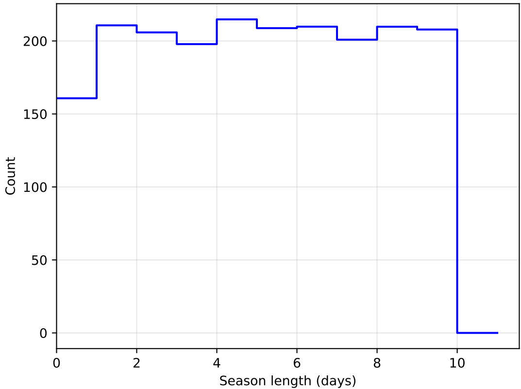
ddf_acor_sf20_lsf40_lsr50_v3.4_10yrs DD:ELAISS1 all bands: SeasonLength
