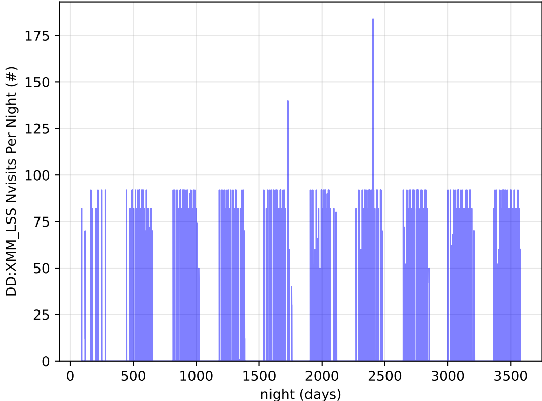
ddf_acor_sf20_lsf40_lsr50_v3.4_10yrs all bands: DD:XMM_LSS Nvisits Per Night
