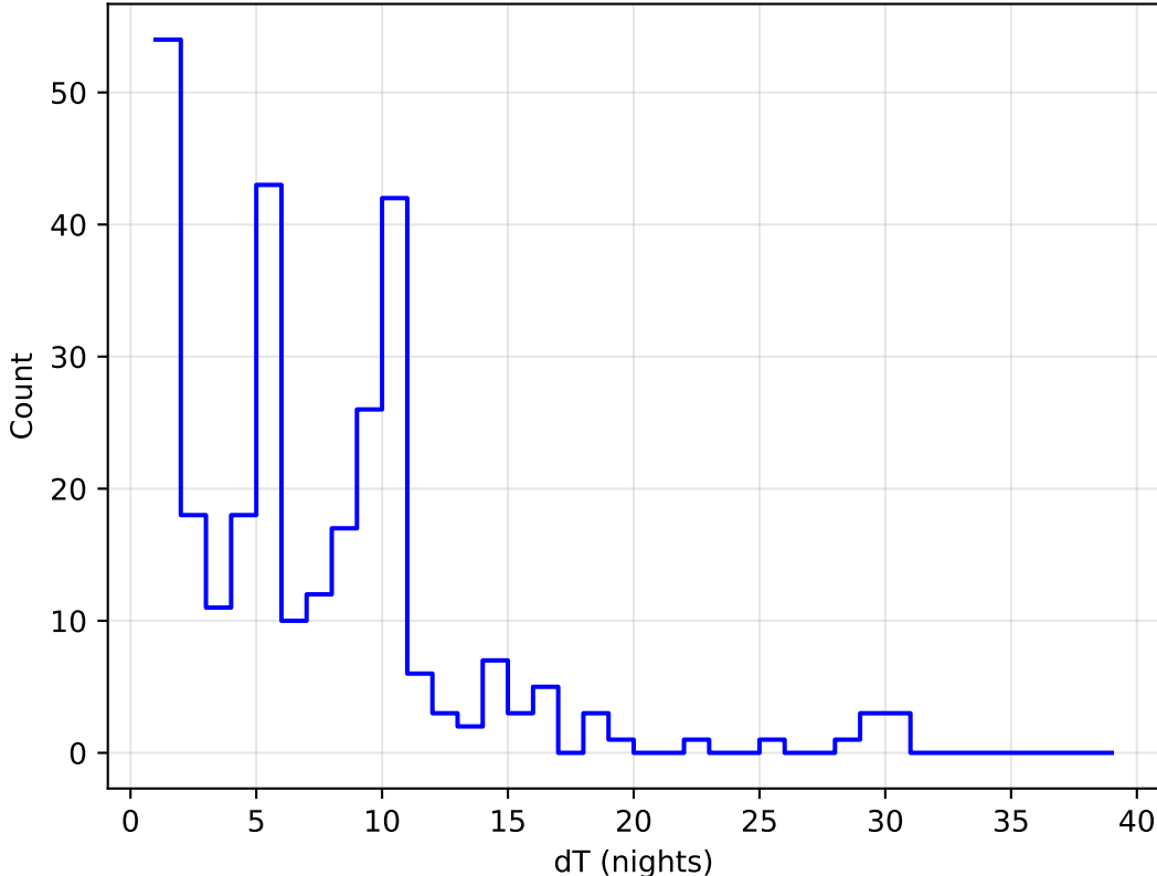
ddf_acor_sf20_Isf40_Isr50_v3.4_10yrs all bands: DD:XMM_LSS Delta Nights Histogram
