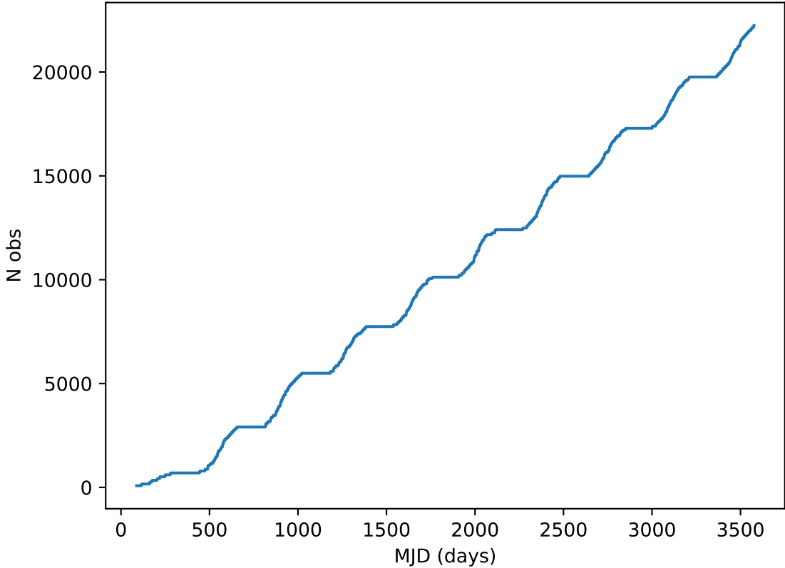
ddf_acor_sf20_lsf40_lsr50_v3.4_10yrs all bands: DD:XMM_LSS Cumulative NVisits
