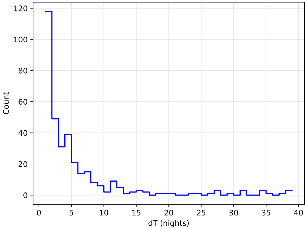
ddf_acor_sf20_lsf40_lsr50_v3.4_10yrs all bands: DD:WFD Delta Nights Histogram
