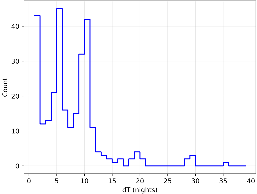
ddf_acor_sf20_lsf40_lsr50_v3.4_10yrs all bands: DD:ELAISS1 Delta Nights Histogram
