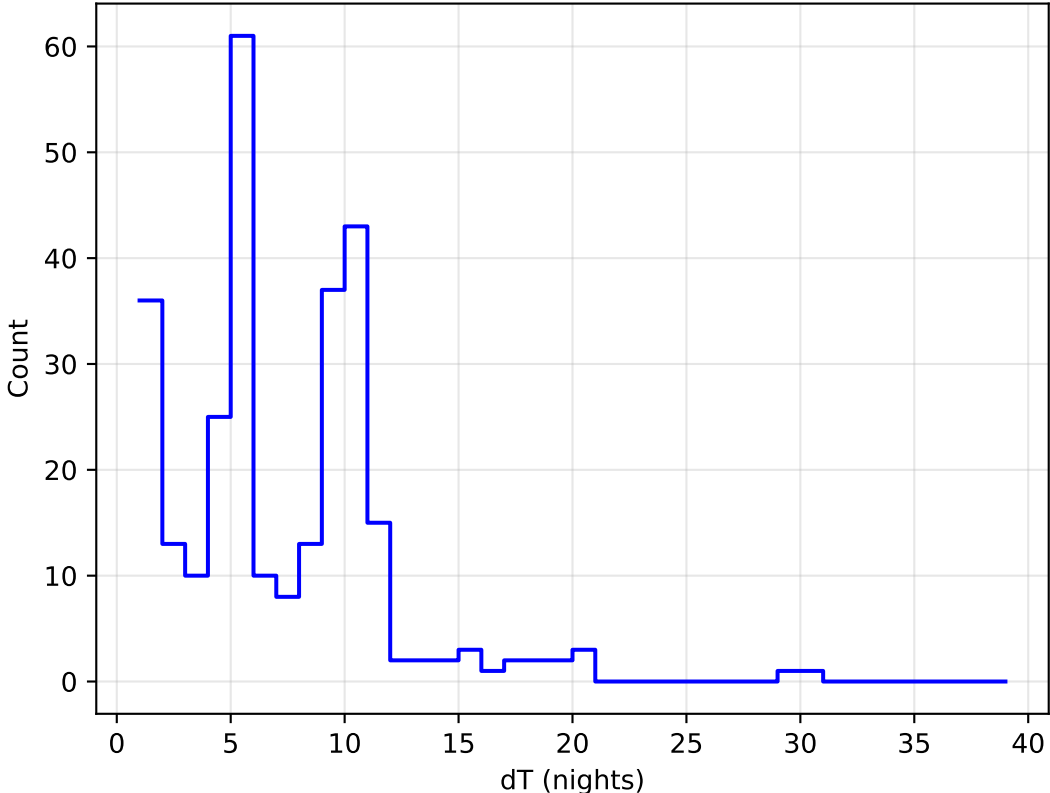
ddf_acor_sf20_Isf40_Isr50_v3.4_10yrs all bands: DD:EDFS Delta Nights Histogram
