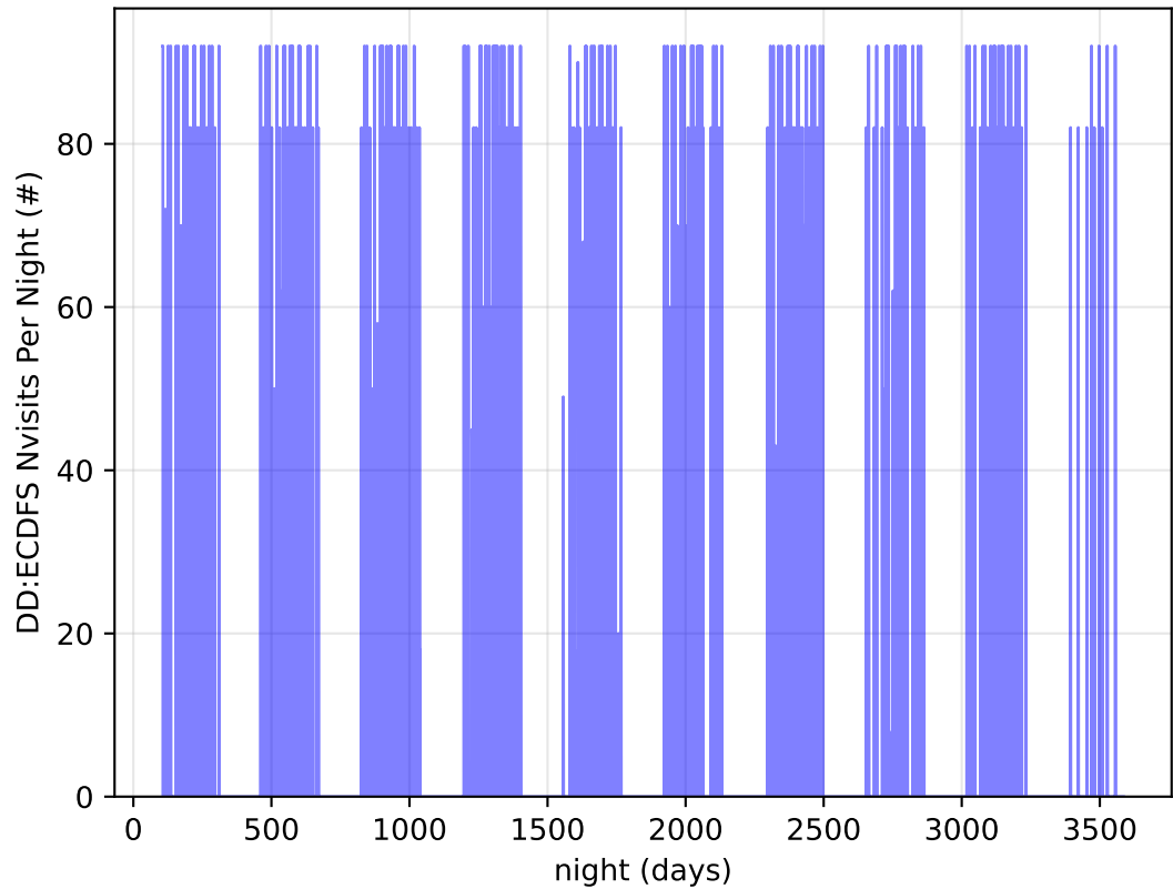
ddf_acor_sf20_ls40_lsr50_v3.4_10yrs all bands: DD:ECDFS Nvisits Per Night
