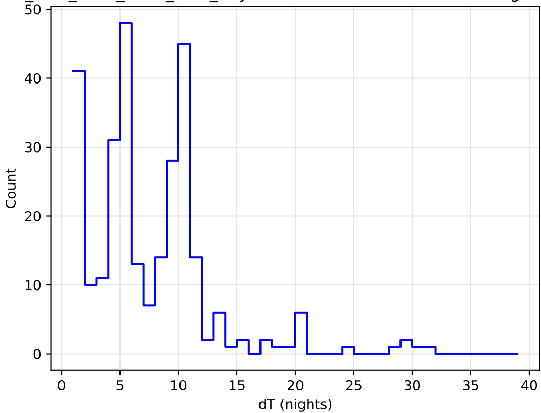
ddf_acor_sf20_lsf40_lsr50_v3.4_10yrs all bands: DD:ECDFS Delta Nights Histogram
