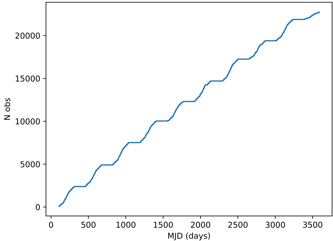
ddf_acor_sf20_lsf40_lsr50_v3.4_10yrs all bands: DD:ECDFS Cumulative NVisits
