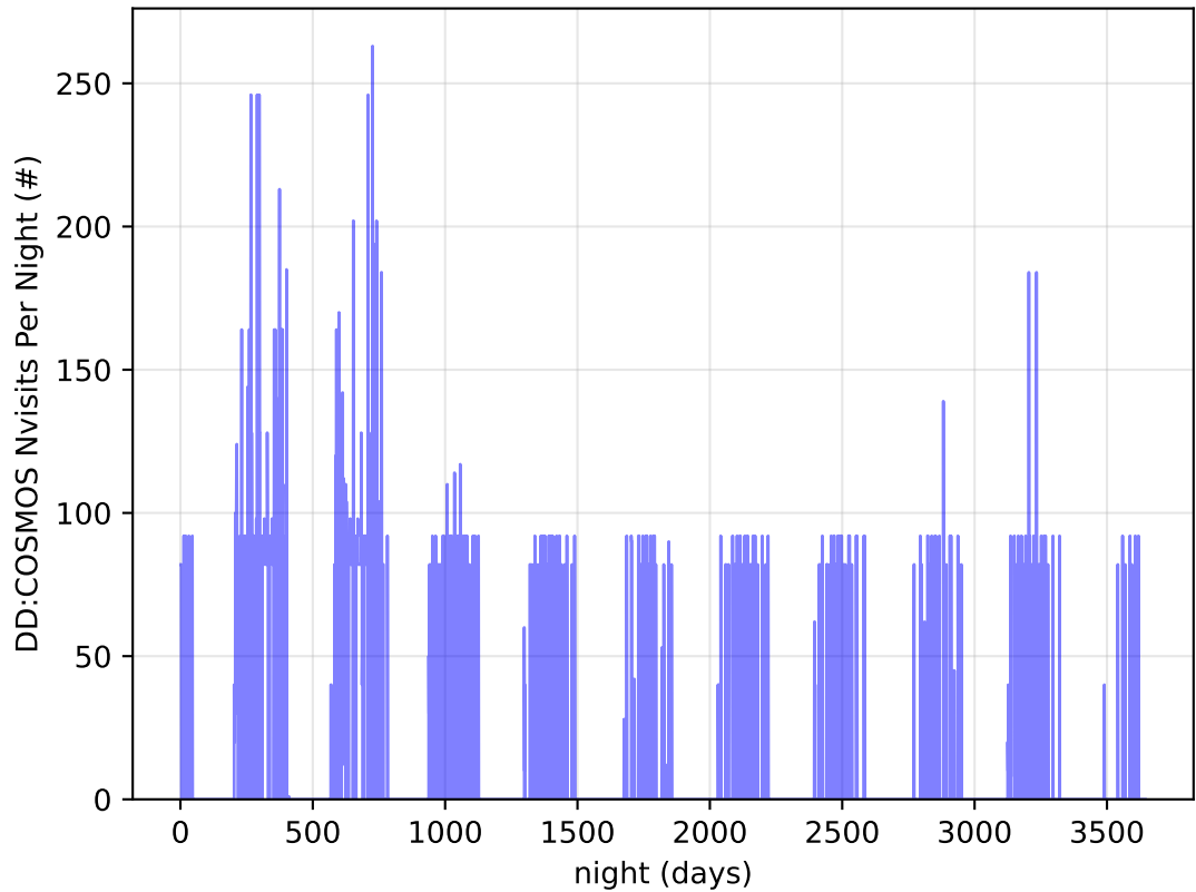
ddf_acor_sf20_lsf40_lsr50_v3.4_10yrs all bands: DD:COSMOS Nvisits Per Night
