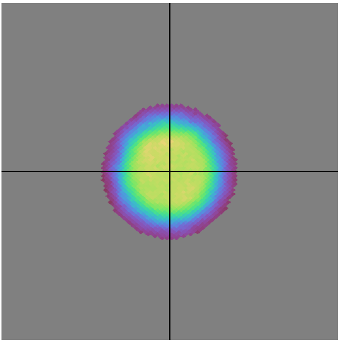
ddf_acor_sf20_lsf40_lsr50_v3.4_10yrs all bands: DD:COSMOS N Unique Nights
