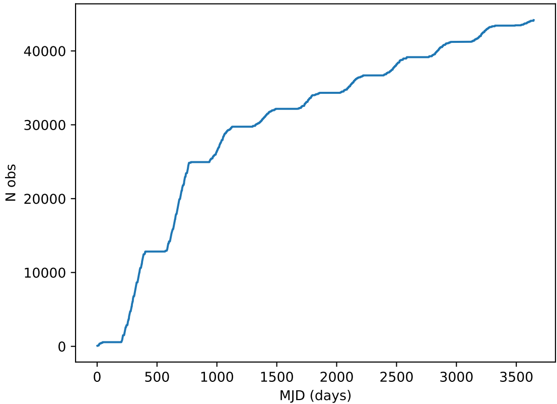
ddf_acor_sf20_lsf40_lsr50_v3.4_10yrs all bands: DD: COSMOS Cumulative NVisits
