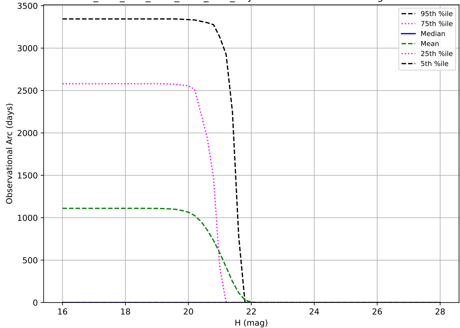
ddf_acor_sf20_lsf40_lsr20_v3.4_10yrs: Observational Arc Length Vatira
