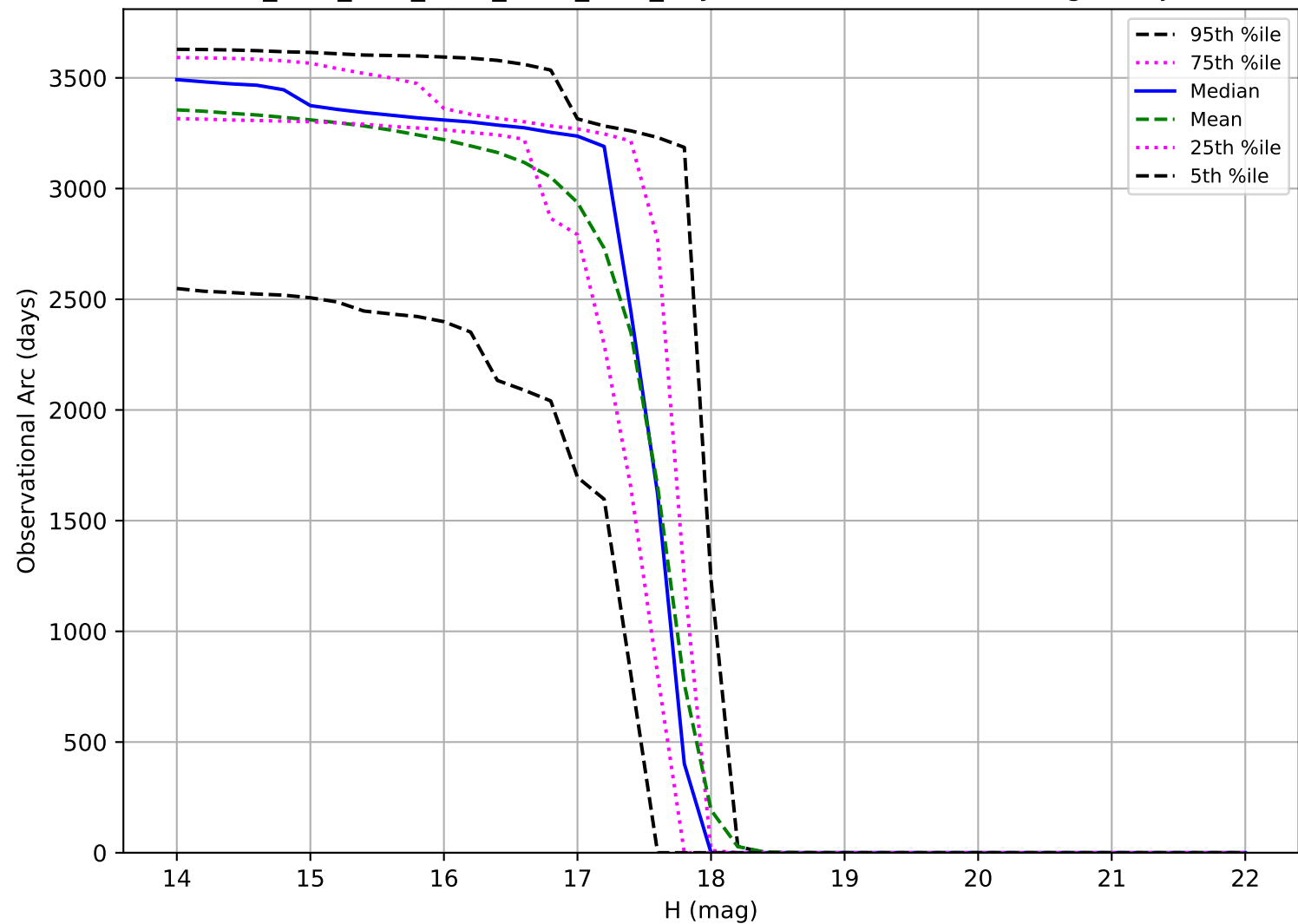
ddf_acor_sf20_lsf40_lsr20_v3.4_10yrs: Observational Arc Length Trojan
