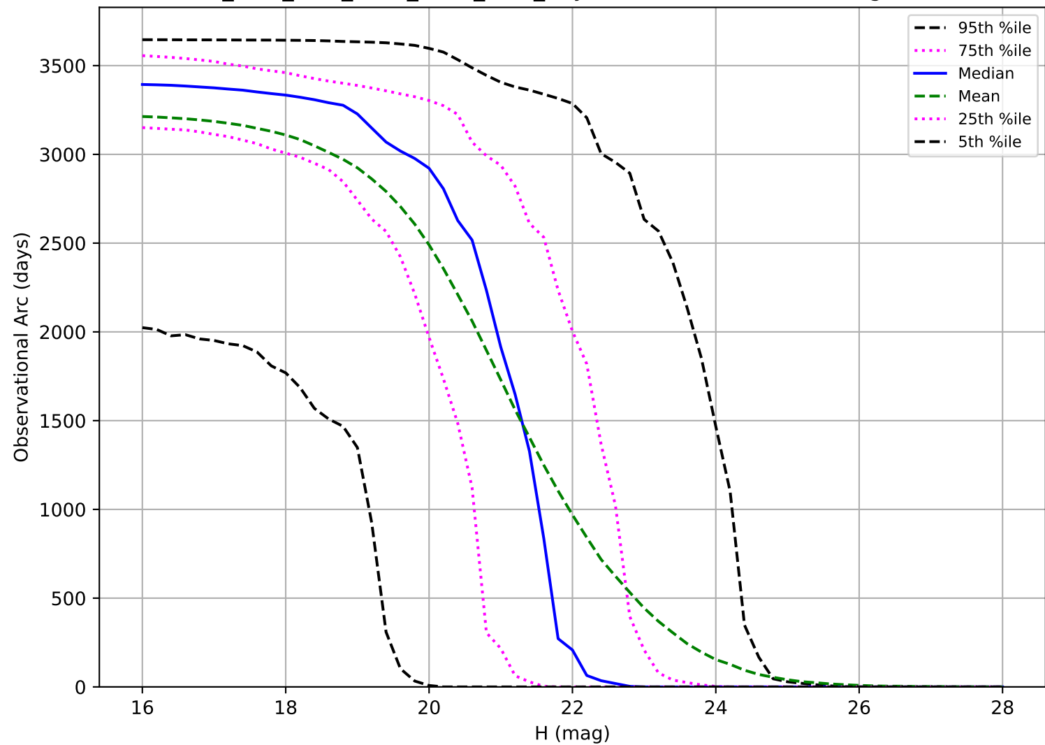
ddf_acor_sf20_lsf40_lsr20_v3.4_10yrs: Observational Arc Length PHA
