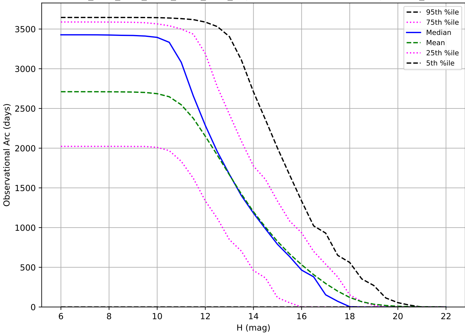
ddf_acor_sf20_lsf40_lsr20_v3.4_10yrs: Observational Arc Length OCC_r5
