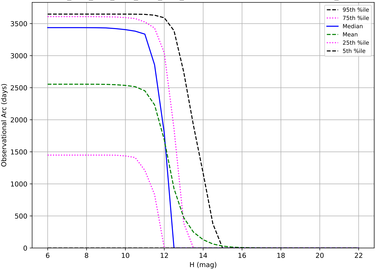
ddf_acor_sf20_lsf40_lsr20_v3.4_10yrs: Observational Arc Length OCC_r20
