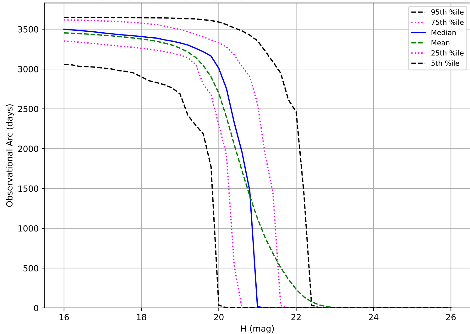
ddf_acor_sf20_lsf40_lsr20_v3.4_10yrs: Observational Arc Length MBA
