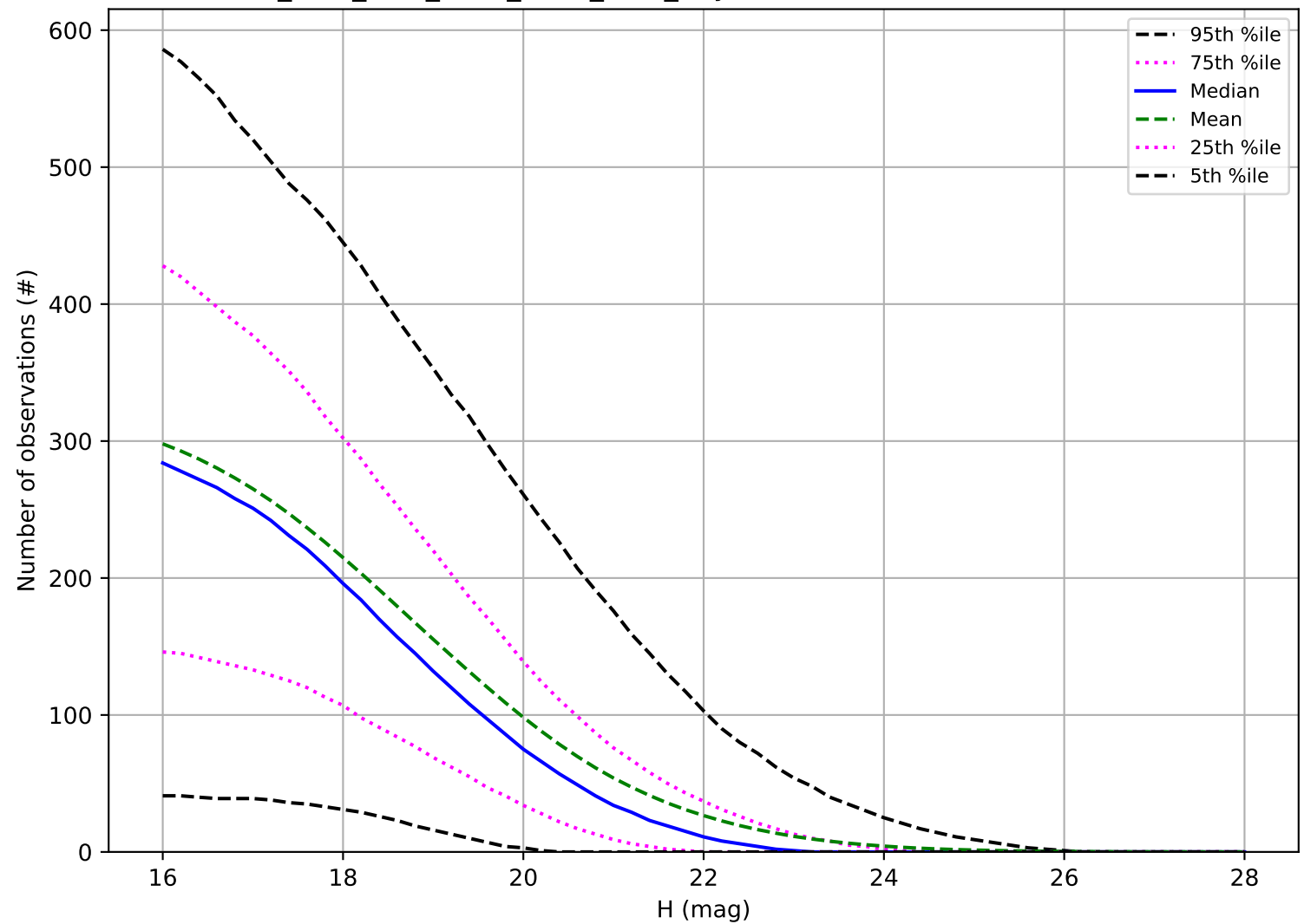
ddf_acor_sf20_lsf40_lsr20_v3.4_10yrs: Number of observations PHA
