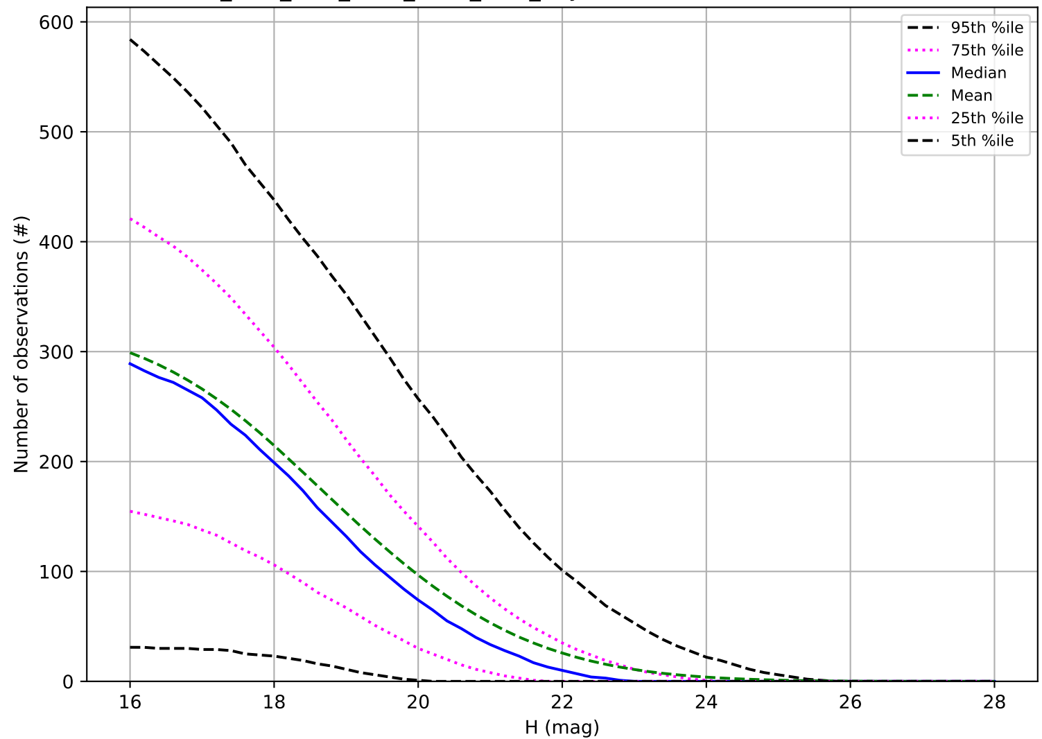
ddf_acor_sf20_lsf40_lsr20_v3.4_10yrs: Number of observations NEO
