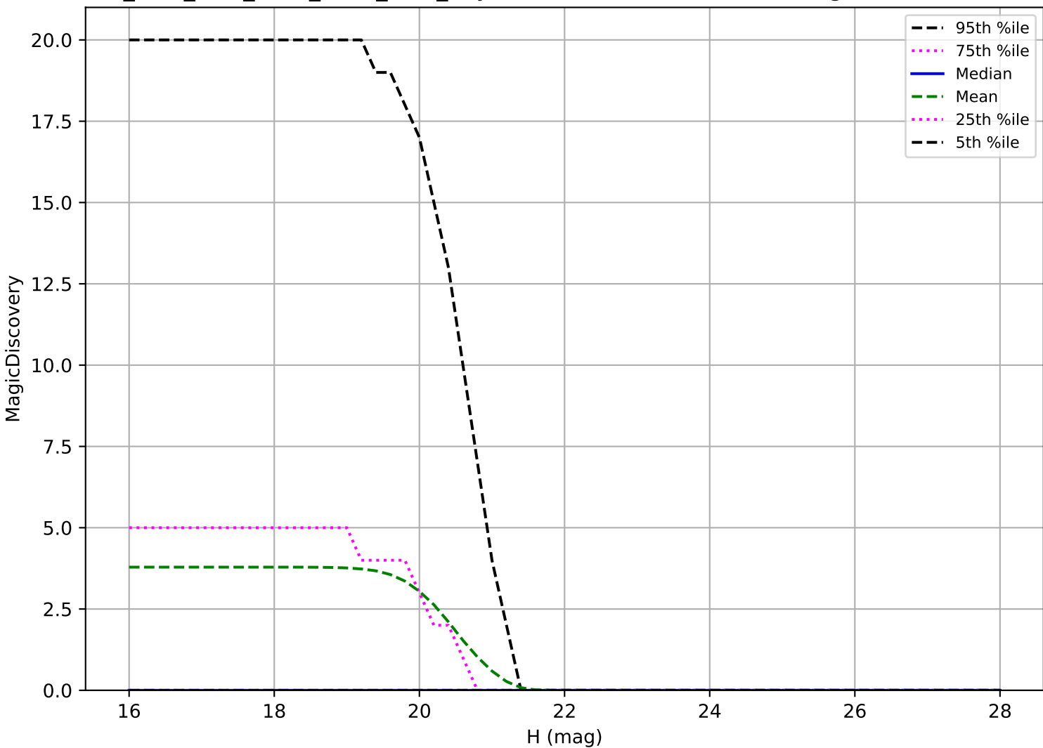
ddf_acor_sf20_lsf40_lsr20_v3.4_10yrs: Vatira 6 detections in 60 nights detection loss
