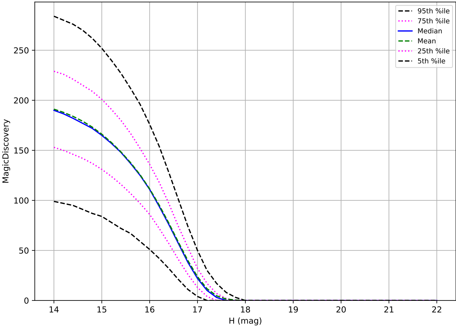
ddf_acor_sf20_lsf40_lsr20_v3.4_10yrs: Trojan 6 detections in 60 nights detection loss
