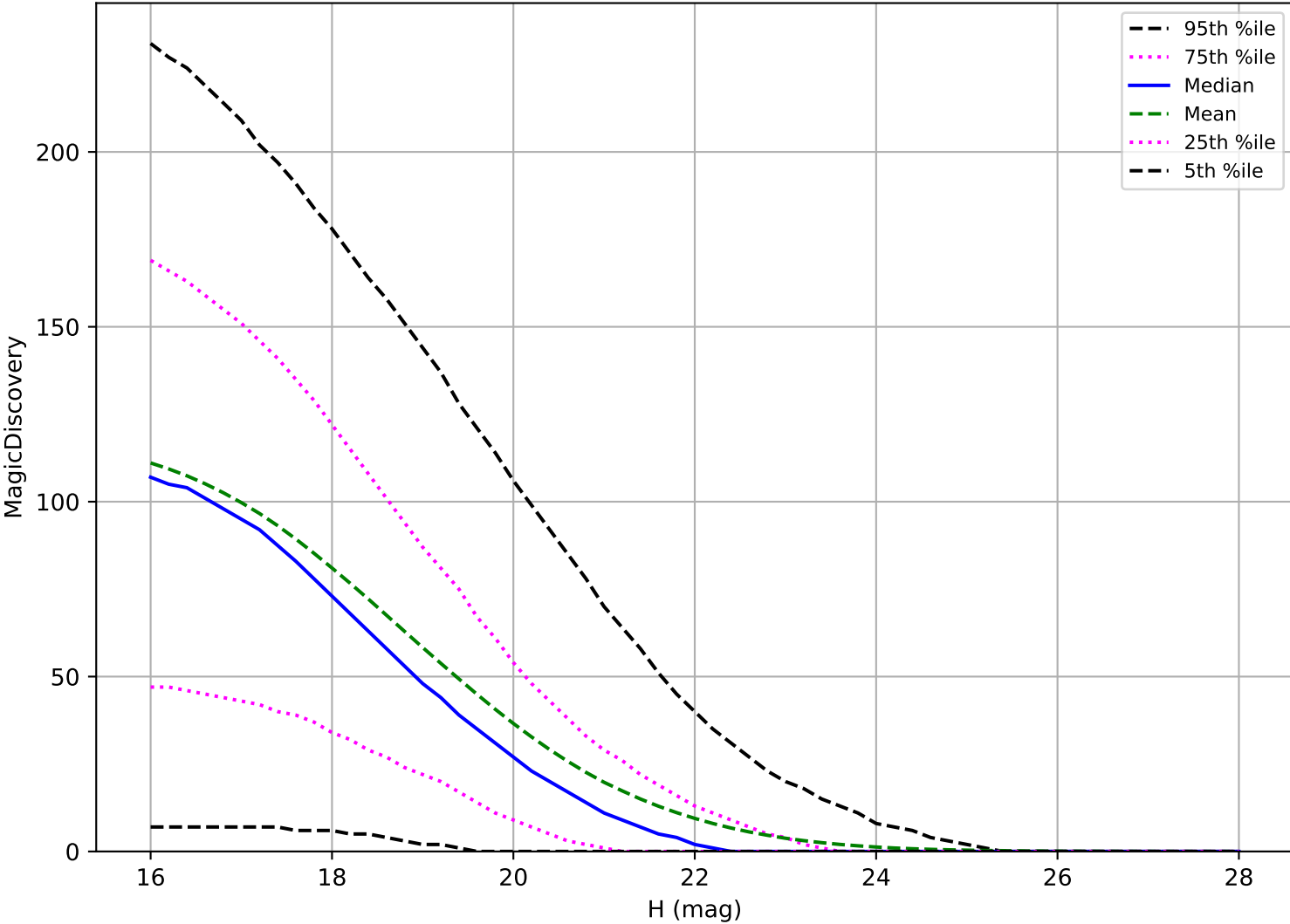
ddf_acor_sf20_lsf40_lsr20_v3.4_10yrs: PHA 6 detections in 60 nights detection loss
