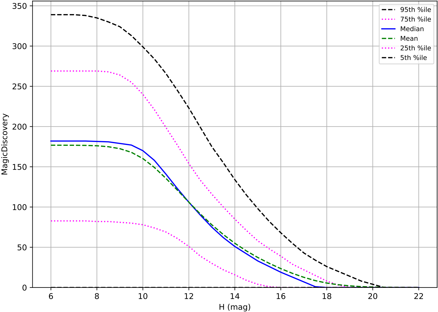
ddf_acor_sf20_lsf40_lsr20_v3.4_10yrs: OCC_r5 6 detections in 60 nights detection loss
