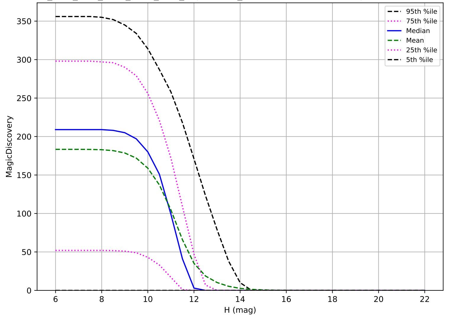
ddf_acor_sf20_lsf40_lsr20_v3.4_10yrs: OCC_r20 6 detections in 60 nights detection loss
