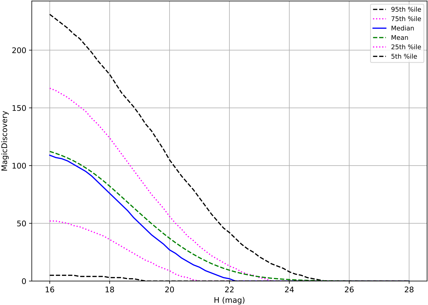
ddf_acor_sf20_lsf40_lsr20_v3.4_10yrs: NEO 6 detections in 60 nights detection loss
