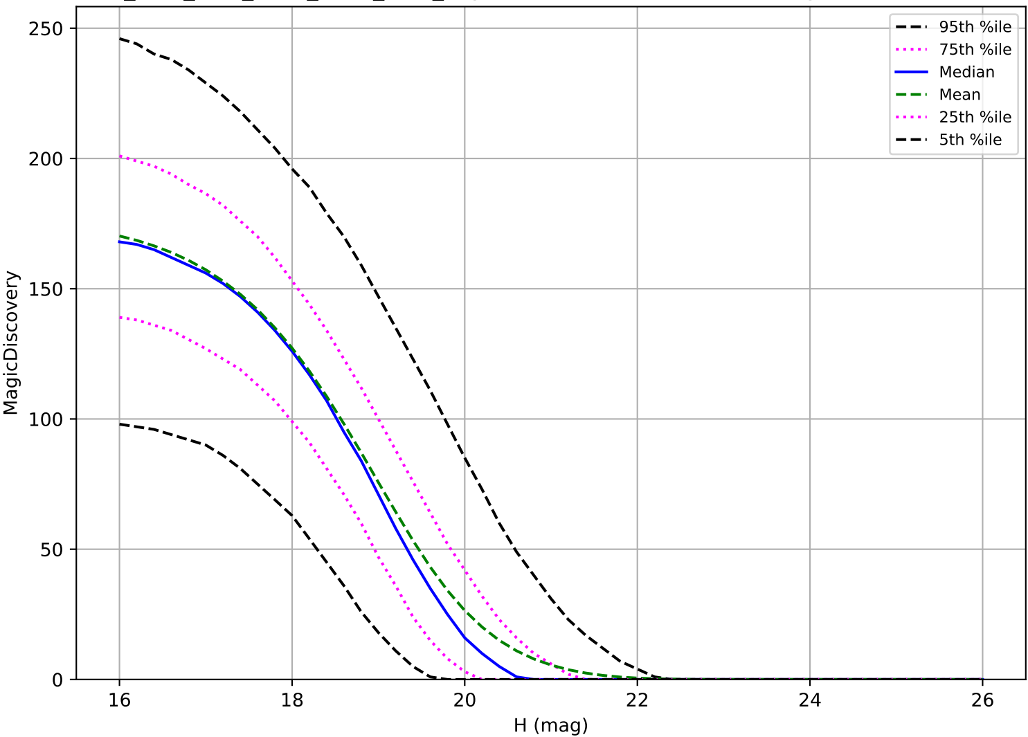
ddf_acor_sf20_lsf40_lsr20_v3.4_10yrs: MBA 6 detections in 60 nights detection loss
