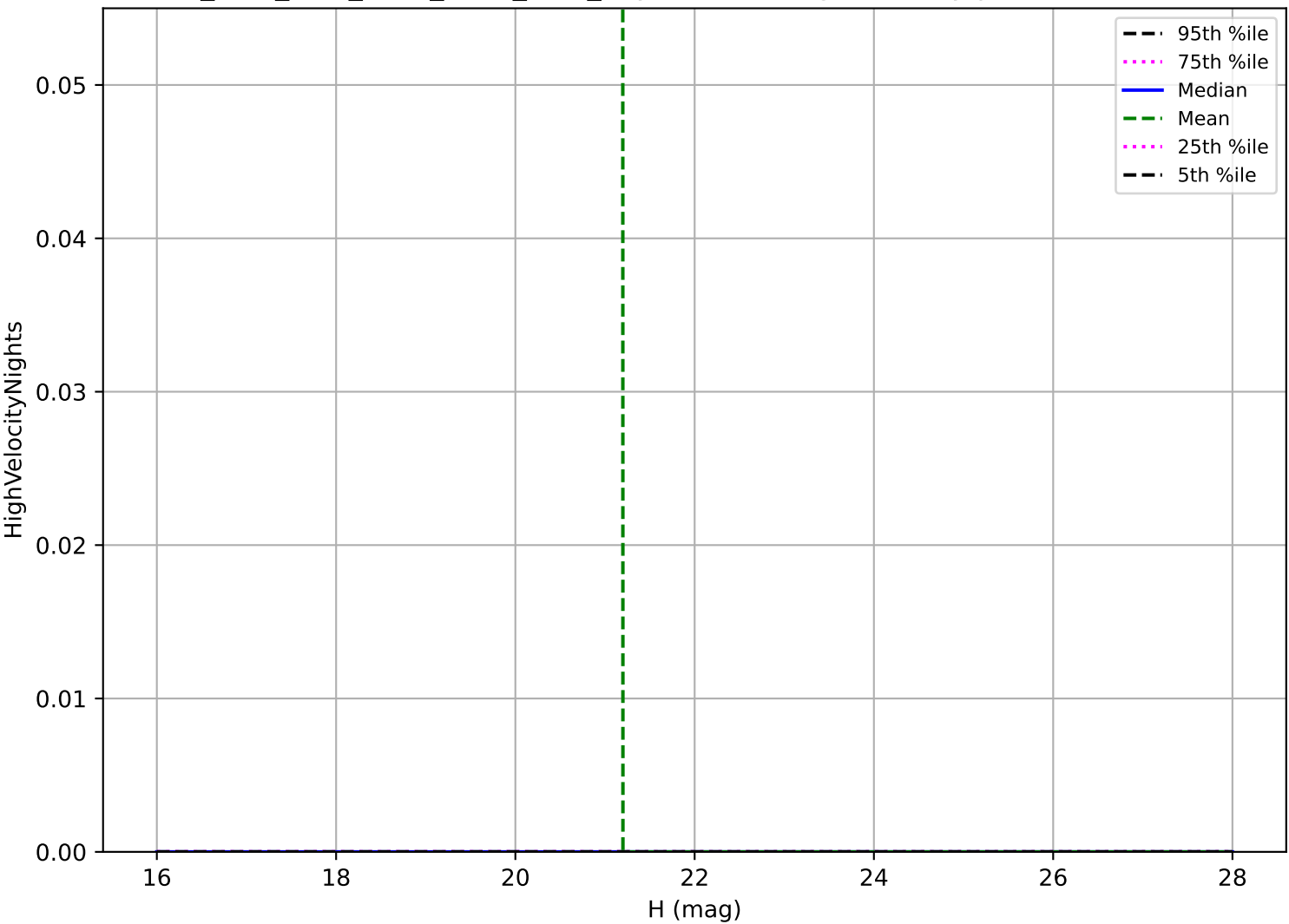
ddf_acor_sf20_lsf40_lsr20_v3.4_10yrs: Vatira High velocity pair detection loss
