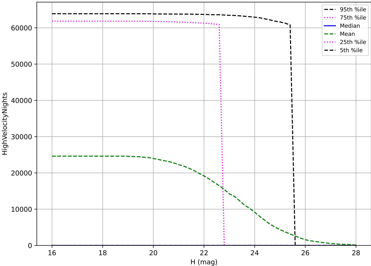
ddf_acor_sf20_lsf40_lsr20_v3.4_10yrs: PHA High velocity pair detection loss
