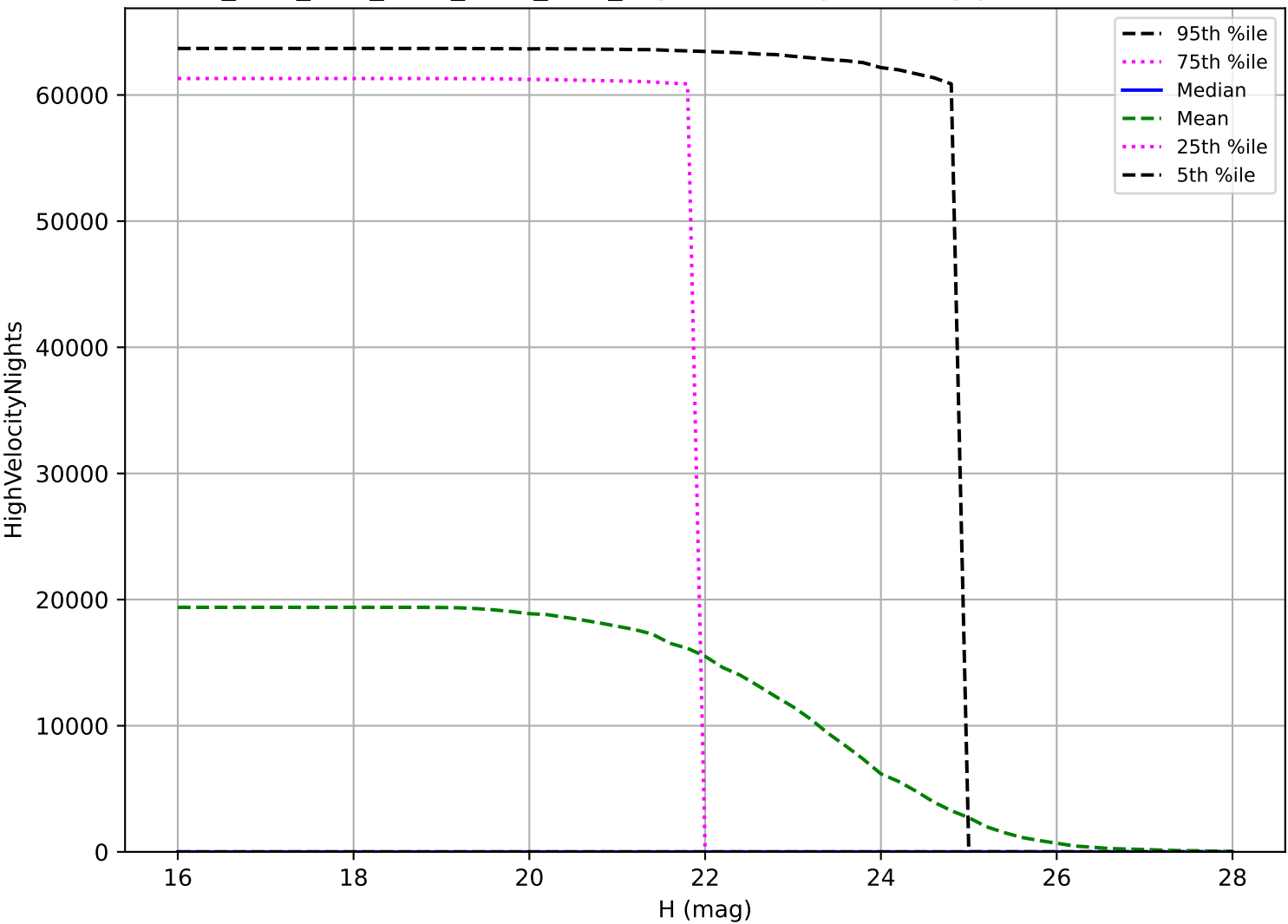
ddf_acor_sf20_lsf40_lsr20_v3.4_10yrs: NEO High velocity pair detection loss
