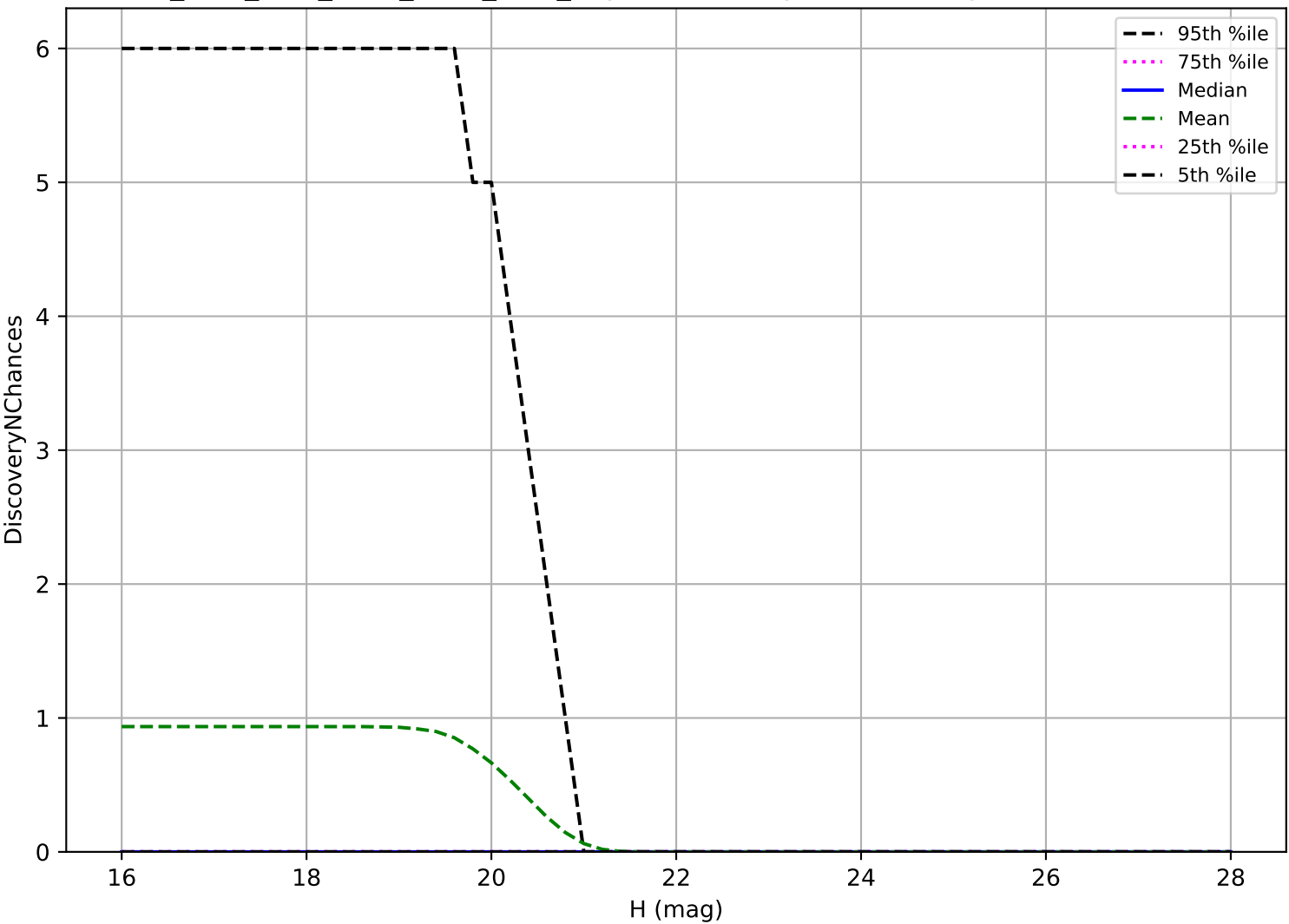
ddf_acor_sf20_lsf40_lsr20_v3.4_10yrs: Vatira 3 pairs in 15 nights detection loss
